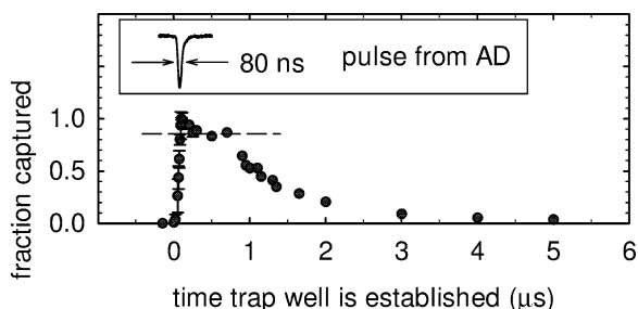
Fig. 4. Number of trapped antiprotons depends upon when the trapping potential is applied.
