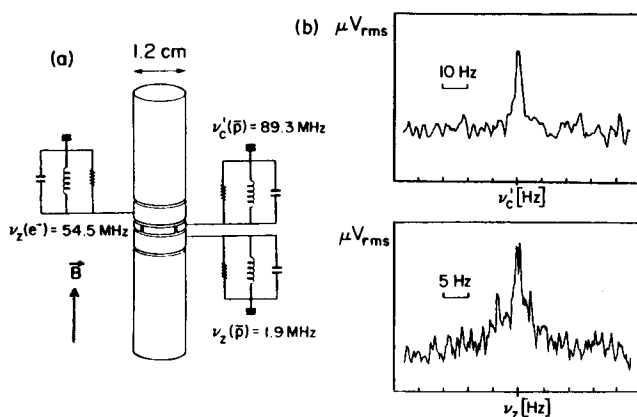
FIG. 2. (a) Trap and ac tuned circuits used to observe the axial motions of electrons (left), the axial motion of antiprotons (lower right), and the cyclotron motion of antiprotons (upper right). (b) Typical antiproton resonances.
