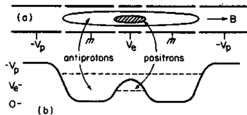
Fig. 1. Electrodes (a) and axial potential (b) for a nested pair of Penning traps.
